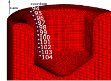
Fig. 5. Data collection on socket region.
