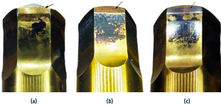
Fig. 7. Surface conditions of TiN coated punches after (a) ~2,000, (b) ~8,000 (arrow shows surface segregation/pitting) and (c) ~10,000 (arrow shows coating removal from surface).
