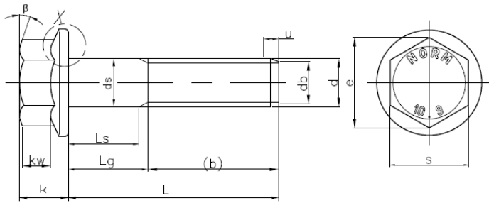
Fig. 1. Drawings of ISO 15071 bolt used in the junker vibration tests.
