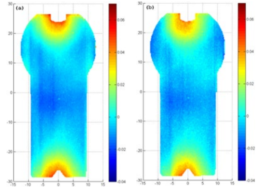
Fig. 7. One of the averaged and gridded contour data of (a) as-forged and (b) subtracted as-forged sample. The axes and the contour plots are in mm.
