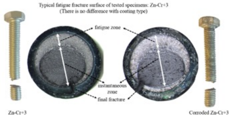
Fig. 5. Fatigue fracture surface of the tested specimen; Zn_{Cr}^{+3} vs corroded Zn_{Cr}^{+3} .
