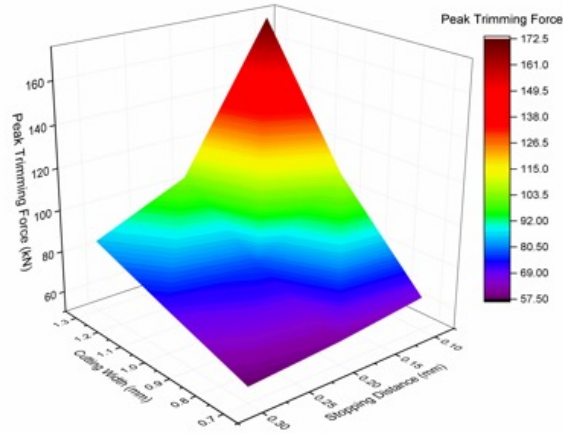
Fig. 13. The relationship between peak trimming load values and CW - SD parameter levels.
