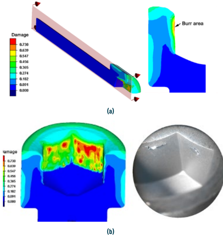
Fig. 4. Distribution of damage in socket area.
