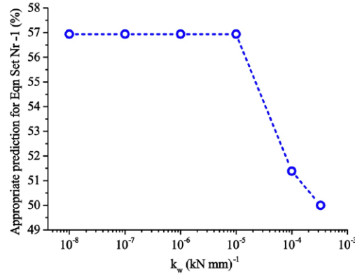
Fig. 6. Change of appropriate prediction percentage with k_w for Eqn. Set Nr-1 of Table 2.
