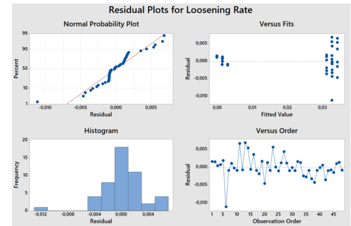
Fig. 5. Residual analysis of loosening rate.
