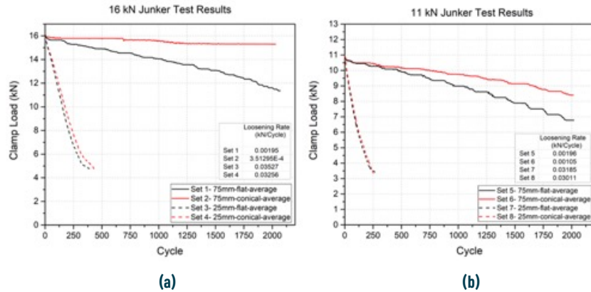
Fig. 4. Junker vibration test results of 16 kN (a) and 11 kN (b).
