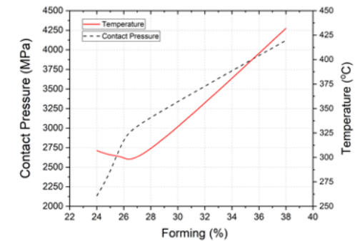
Fig. 3. Variation of contact pressure and forming temperature during forging.
