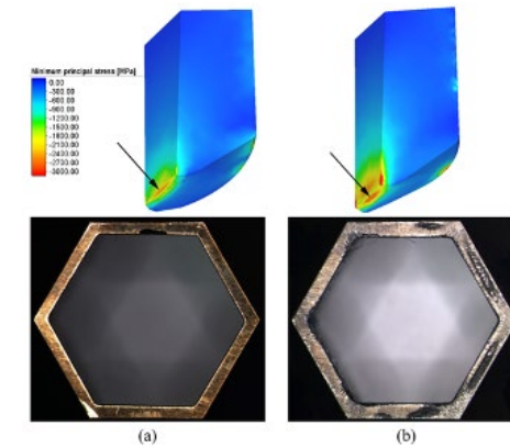
Fig. 9. Minimum principal stresses occurred on the edge radius and cutting width part: a) Cutting Width: 0.7 mm; b) Cutting Width: 1.1 mm.
