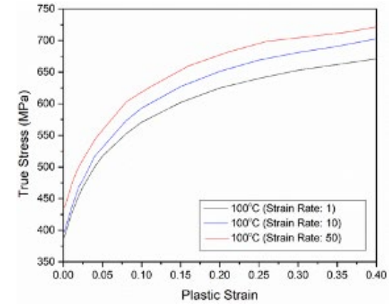
Fig. 2. Experimental flow curves for a medium carbon alloy steel material at different strain rates for 100 °C.
