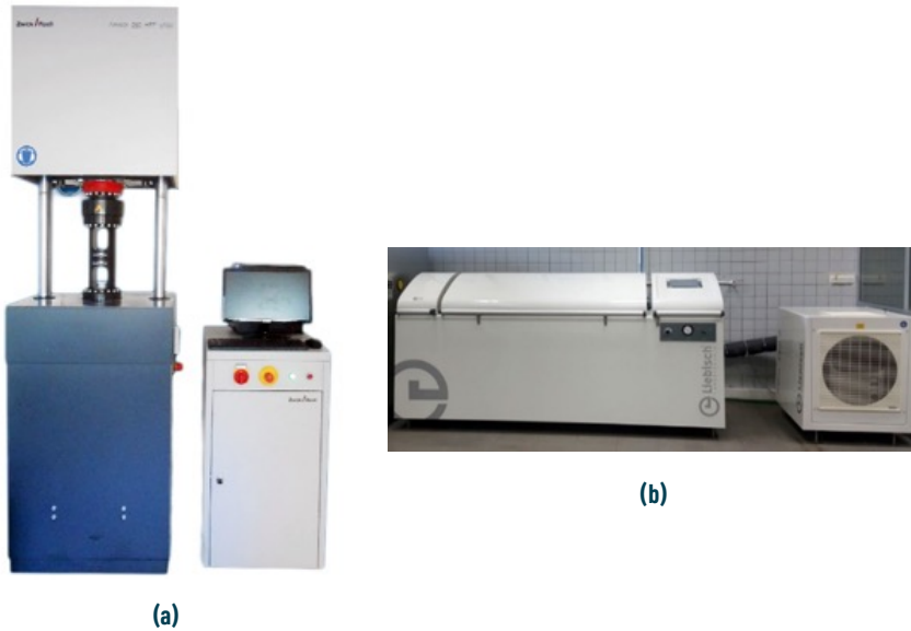
Fig. 2. Test equipments; (a) Axial load fatigue and (b) salt spray testing chamber.
