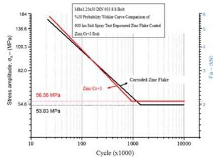
Fig. 10. Fatigue life comparison of Zinc flake bolts after corrosion test and Zn\text{-}Cr^{+3} coated bolts.
