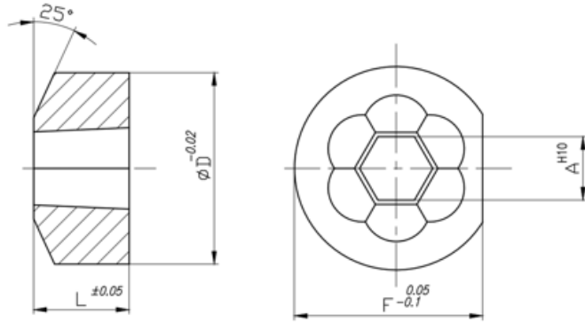
Fig. 2. Technical drawing of trimming die.
