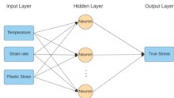
Fig. 3. The schema of constructed ANN model.
