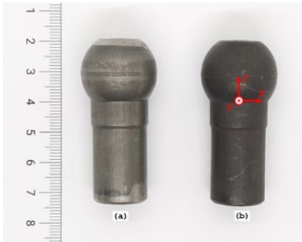
Fig. 2. (a) As-forged and (b) heat-treated ball studs used in this study. (y=0 is the mid-thickness of the ball stud)
