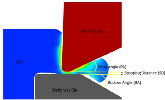
Fig. 5. Design parameters of trimming process.
