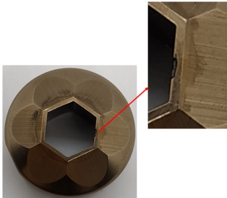
Fig. 6. Chips occurrence on the reference trimming die.
