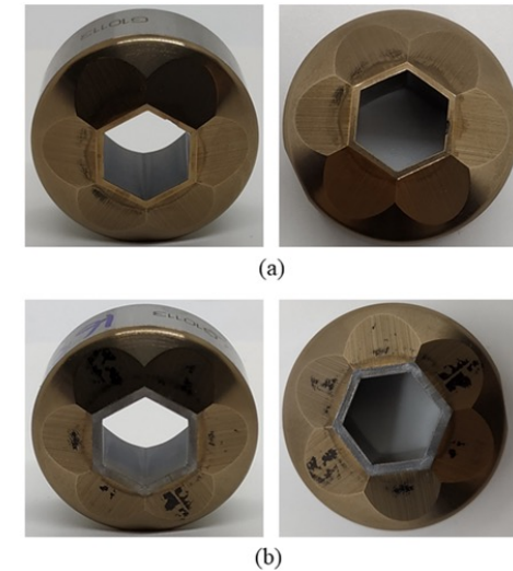
Fig. 1. Examples of hexagonal trimming dies before and after grinding operation: a) Before; b) After.
