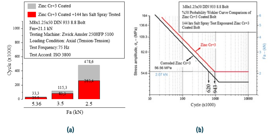
Fig. 7. (a) Fatigue tests results and (b) Wöhler curves of Zn_{Cr}^{+3} coated bolts before and after salt spray tests.
