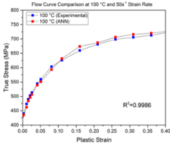
Fig. 7. Comparison of ANN predictions for the validation data set, strain rate: 50 \text{ s}^{-1} .
