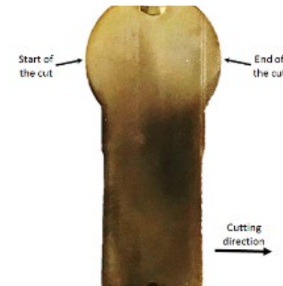
Fig. 5. One of the cut surfaces of as-forged sample. The height of the ball stud is 56 mm.
