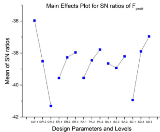
Fig. 11. Main effect plot for the peak trimming load objective function.
