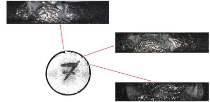
Fig. 2. Surface cracks and their locations of two different shot peened samples subjected to compression tests.
