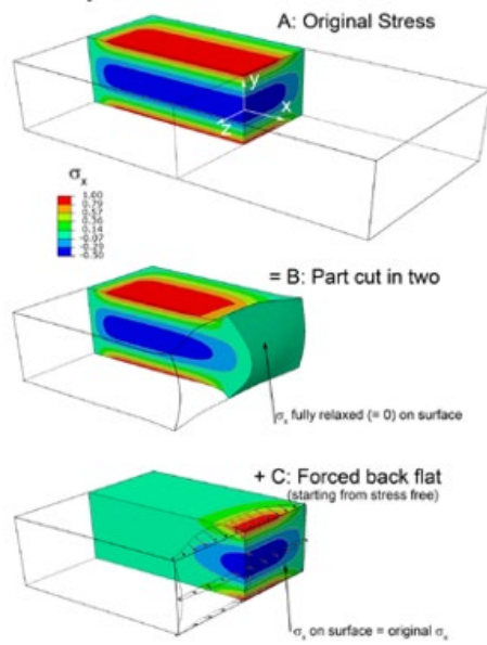
Fig. 3. Superposition Principle employed for the contour method. Only quarter of the sample is plotted [20].
