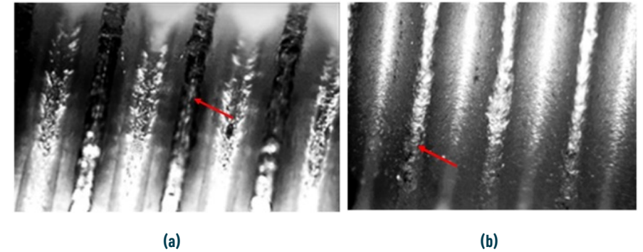
Fig. 3. Pictures of thread roots; a) Zn_{Cr^{+3}} , b) Zinc flake [13].
