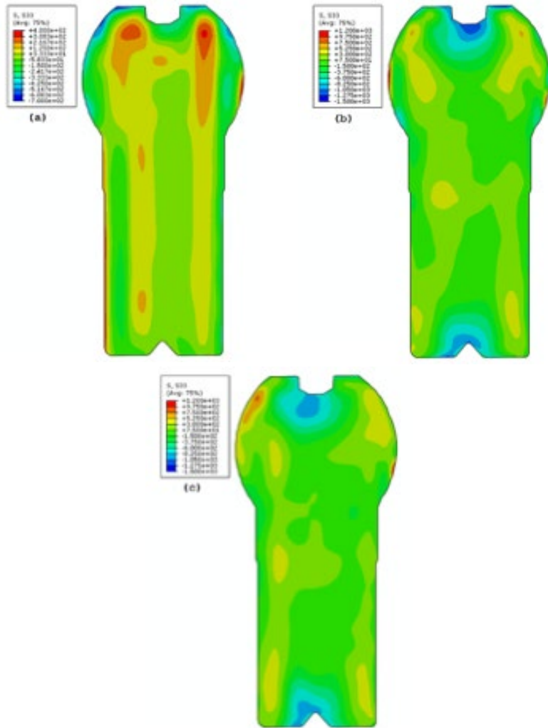
Fig. 8. 2D residual stress maps of (a) heat-treated, (b) as-forged and (c) subtracted as-forged samples. Scale for residual stresses given in (a) is different than (b) and (c). Scales are the same for (b) and (c).
