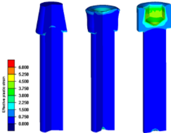
Fig. 1. Numerical representation of forging steps of a bolt having internal socket.
