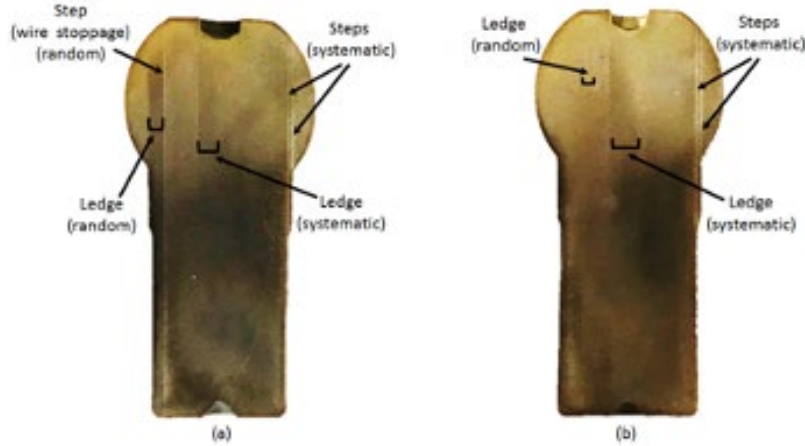
Fig. 11. Systematic and random cutting-induced artefacts for (a) heat-treated and (b) as-forged sample.
