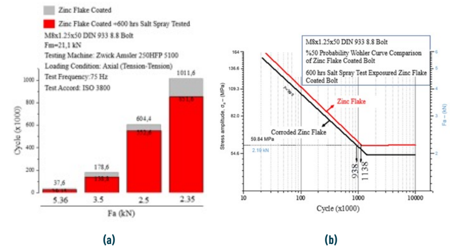
Fig. 8. (a) Fatigue tests results and (b) Wöhler curves of Zinc flake coated bolts before and after salt spray tests.
