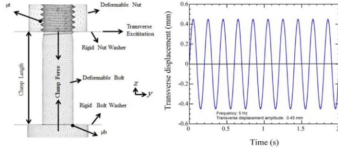
Fig. 3. Finite element model of bolted-joint and applied transverse displacement versus time curve.
