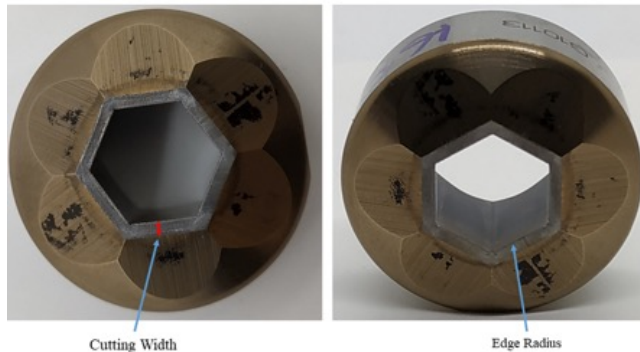
Fig. 3. The cutting width and edge radius measurements on the trimming die.
