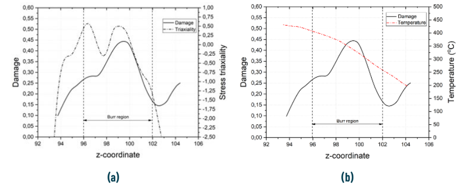
Fig. 6. Variation of damage, stress triaxiality and temperature in the socket region.
