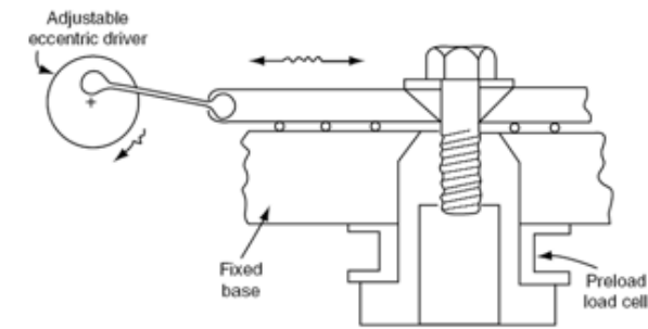
Fig. 3. The Junker vibration test device (Bickford, 2008).
