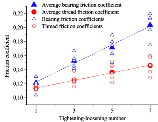
Fig. 4. The variations of the thread and bearing friction coefficients with the number of tightening-loosening.
