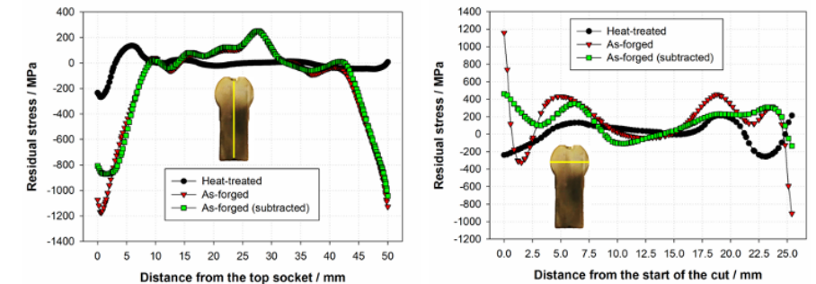
Fig. 9. Line profiles of heat-treated and forged samples. Location of the residual stresses was shown in the figure.
