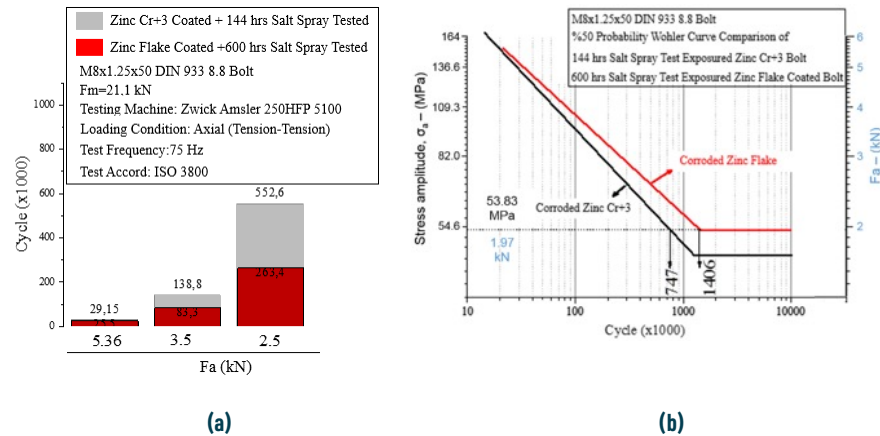
Fig. 9. Comparison of (a) Fatigue tests results and (b) Wöhler curves of Zinc flake and Zn\text{-}Cr^{+3} coated bolts after salt spray tests.
