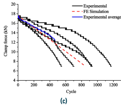
Fig. 7. The curves of numerical simulation results of (a) M_t versus transverse displacement and (b) F_s versus transverse displacement and (c) the experimental and FE model clamp force versus cycle.
