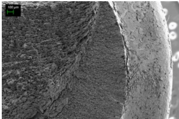
Fig. 6. SEM image of fracture surface of the tested specimen.
