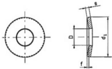
Fig. 2. Drawings of the conical washer used in vibration tests.
