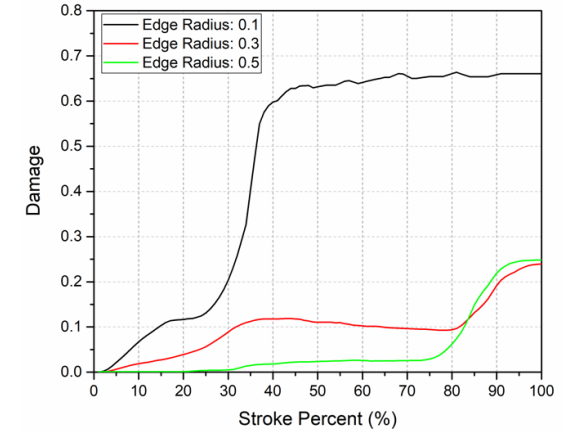
Fig. 14. Damage - stroke graph for all levels of ER parameter.
