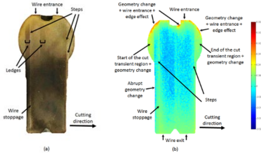
Fig. 6. (a) One of the cut surfaces and (b) averaged and gridded contour data of heat-treated sample. The contour plot is in mm.
