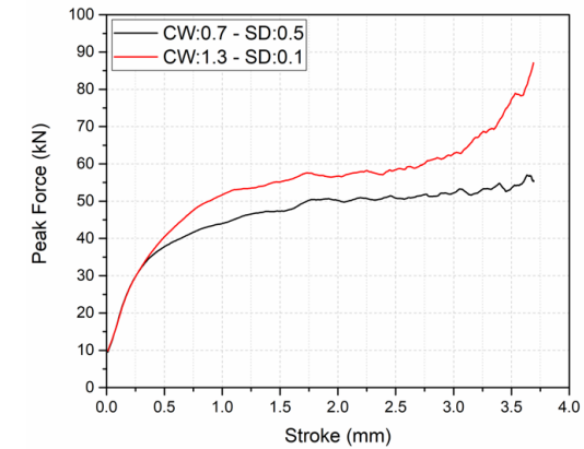
Fig. 12. Trimming force - stroke for the best and worst levels of CW and SD parameters.
