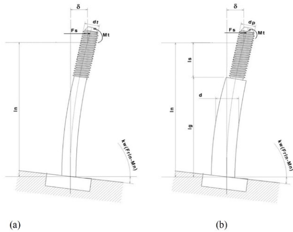
Fig. 1. (a) Deflection of a bolt caused by a transverse external force and (b) deflection of multi sectioned bolt caused by transverse external force.
