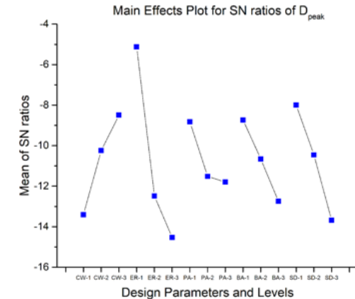
Fig. 15. Main effect plot for the peak damage value objective function.
