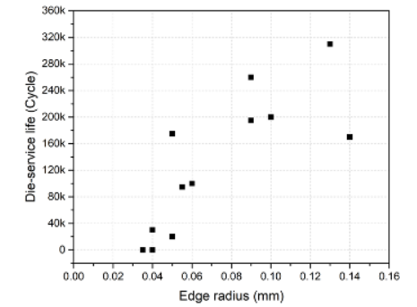
Fig. 8. Graph of edge radius versus die-service life.
