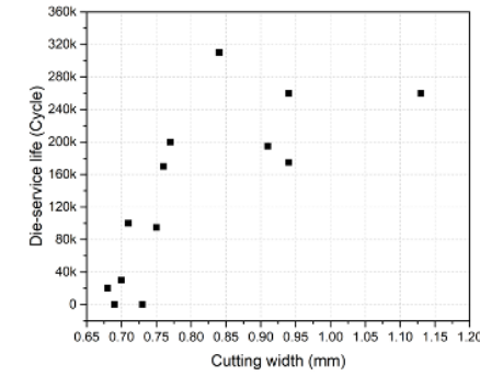
Fig. 7. Graph of cutting width versus die-service life.
