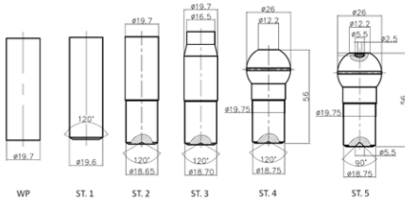
Fig. 1. Cold forging stage designs and final dimensions of ball studs.
